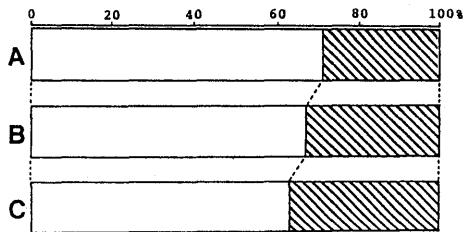
Fig. 2. Comparison of anthocyanin contents, delphinidin 3-rutinoside (□) and cyanidin 3-rutinoside (▨), in blue (var. udensis , A), intermediate (B) and black ( f. nigra , C) pericarps of Clintonia udensis .
